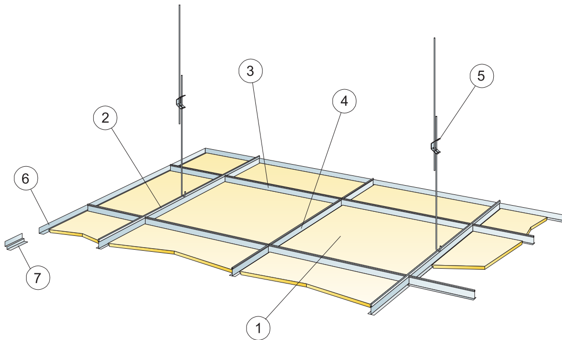
Installation diagram (M140) for Ecophon Opta E
